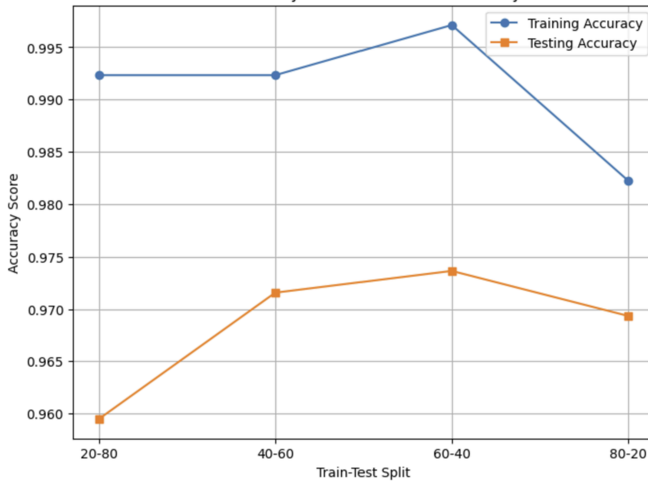
Chest X-Ray CNN: Train vs Test Accuracy
